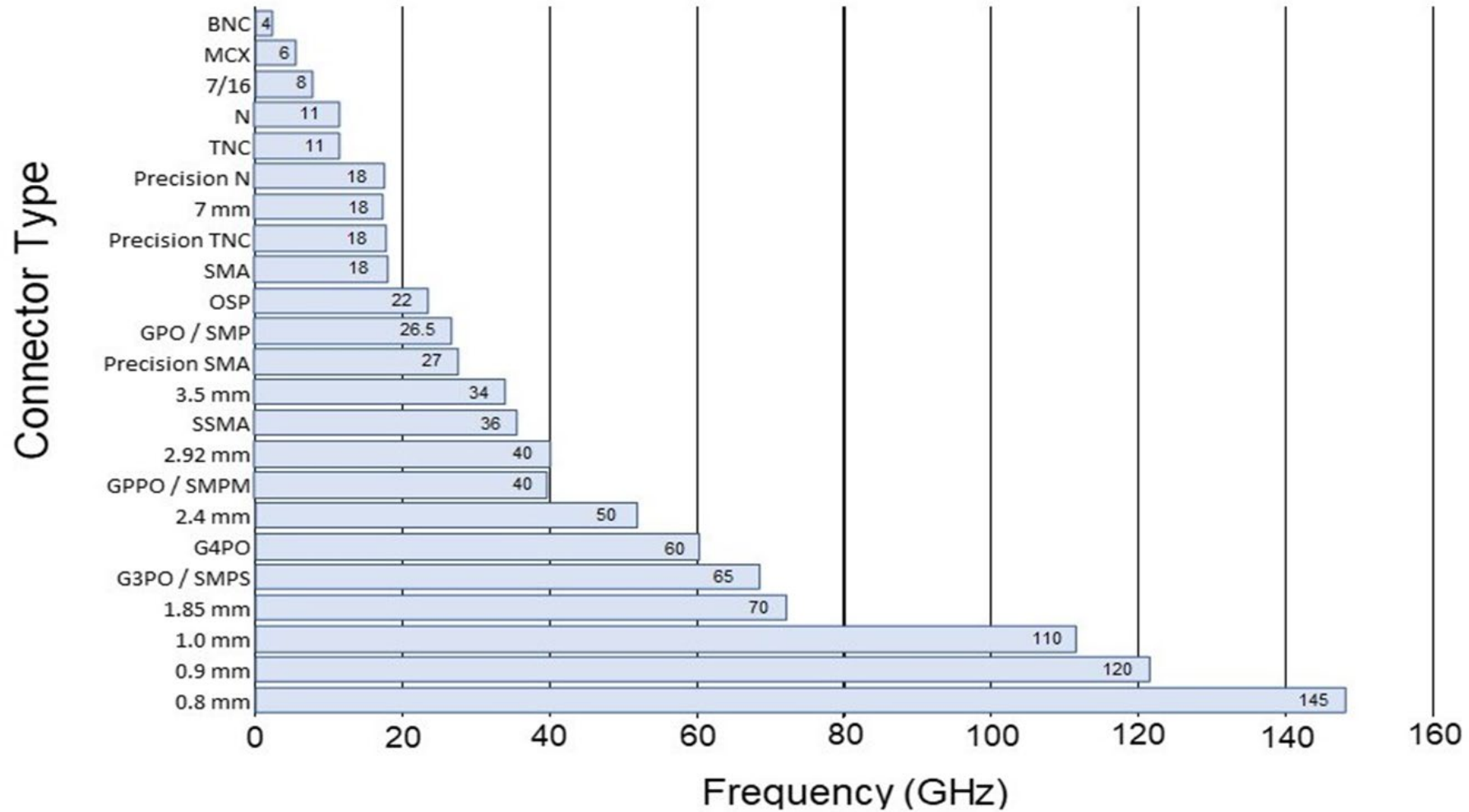
50 Ohm Coax Connector Frequency Limitations
